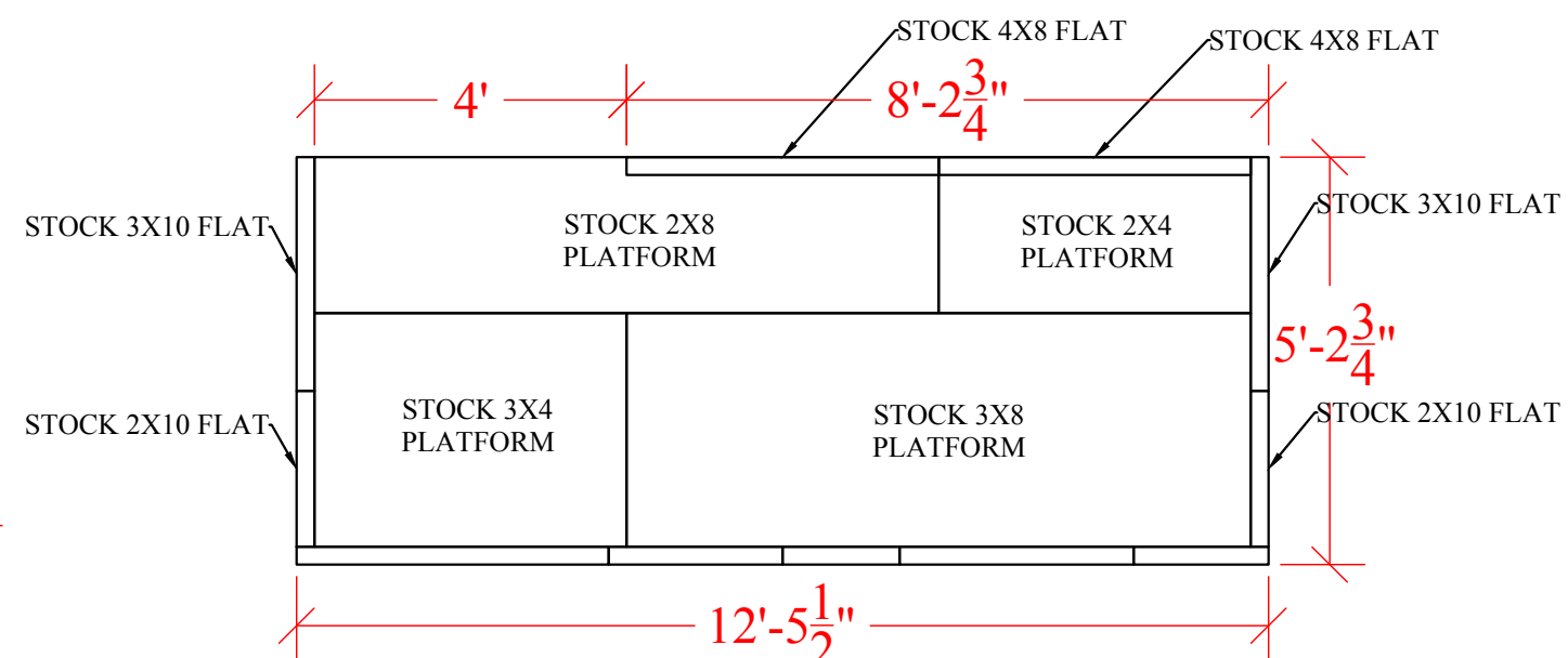
SECTION B-B
