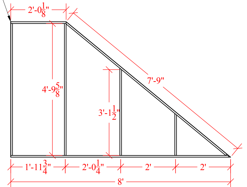
1x4 HOLLYWOOD FLAT FRAMING FRONT VIEW
