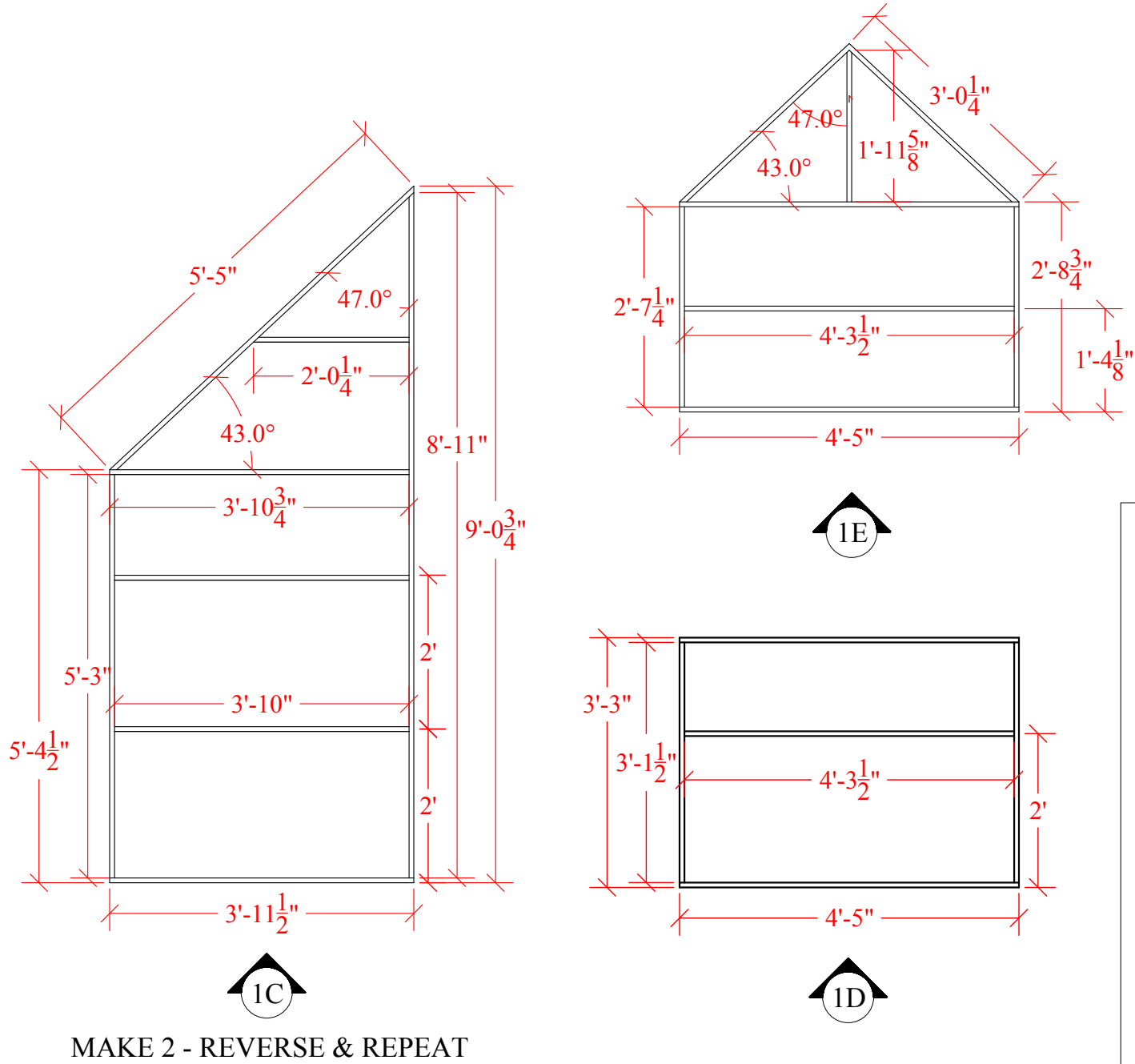
1x3 HOLLYWOOD FLAT FRAMING SCALE: \frac{1}{2}" = 1'-0"
