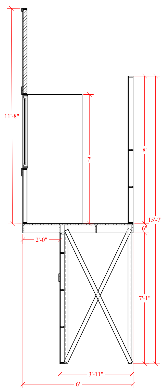
SECTION C-C
