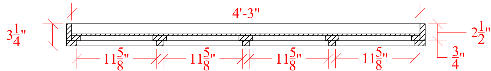
SECTION B-B
