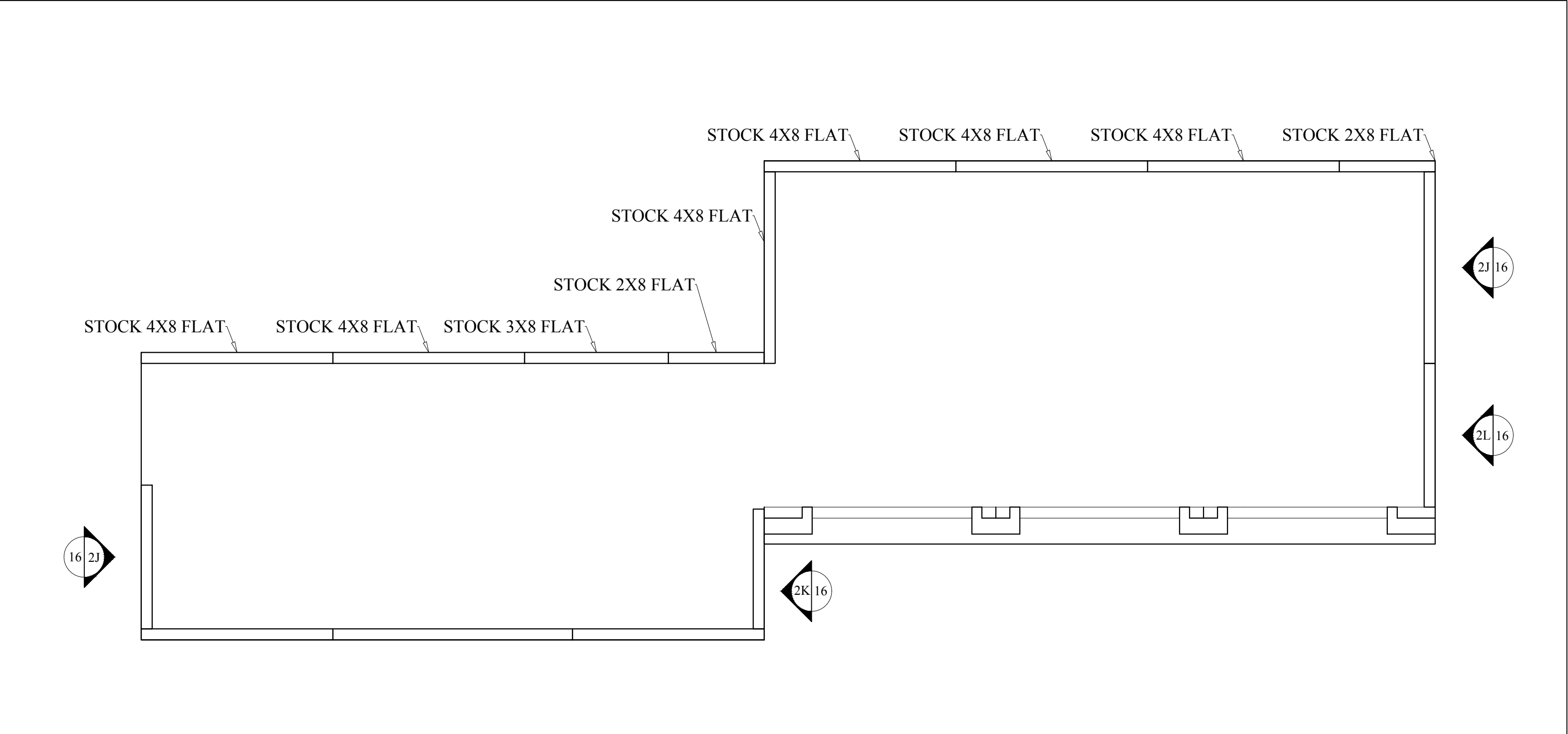
SECTION B-B
